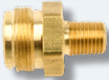
Model F173755 Propane 1"-20 Male Throwaway Cylinder Thread x 1/4" Male Pipe Thread (bulk available -73755)
