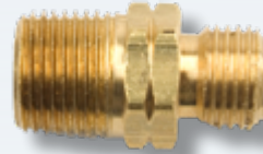
Model F176153 3/8" Male Pipe Thread x 9/16" Left Hand Male Thread (bulk available -76153)
