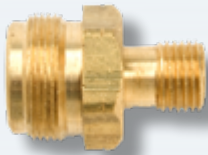
Model F176130 Propane 1"-20 Male Throwaway Cylinder Thread x 9/16" Left Hand Male Thread w/ Shut-off
